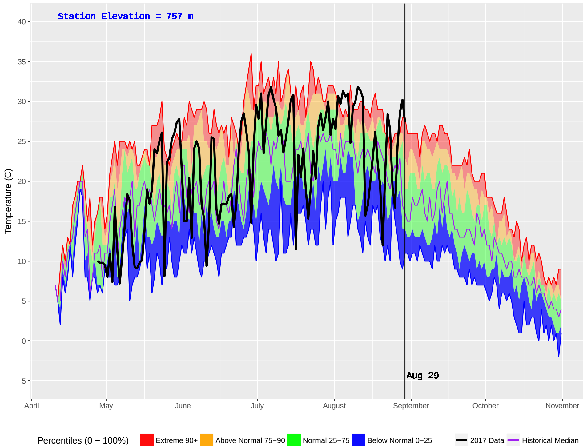
DOWNIE (905) : Historical (2005–2016) and Current (2017) Noon Temperature
