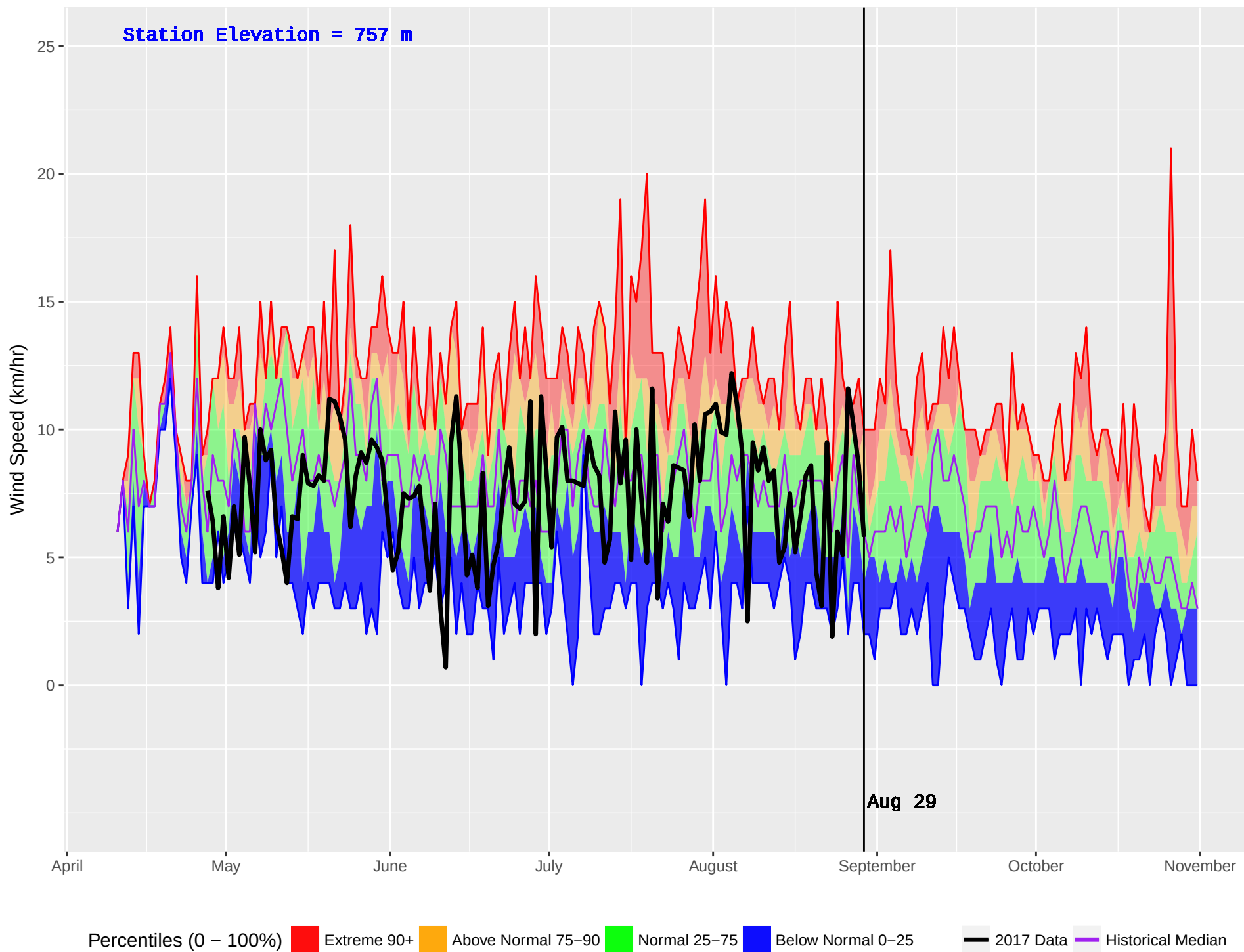
DOWNIE (905) : Historical (2005–2016) and Current (2017) Noon Wind Speed
